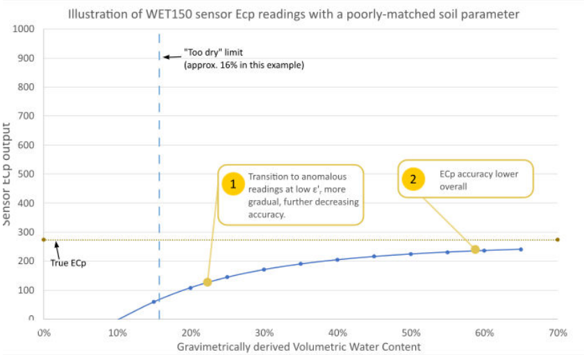
Figure 3 - Illustration of how sensor ECp output is affected by a poorly-matched soil parameter. Note that although this illustration tends to negative infinity, either positive or negative infinity asymptotes are possible
