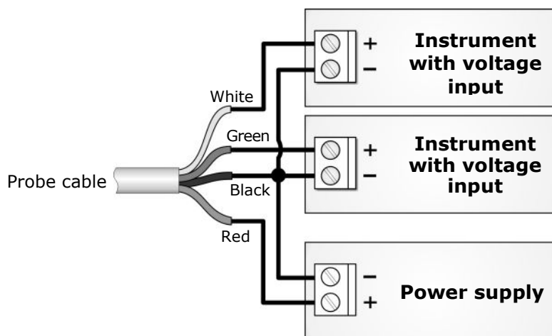
Fig. 4: analog outputs connection
